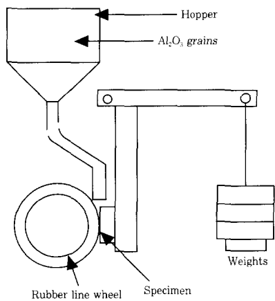
Fig. 2 Schematic of abrasive erosion test
