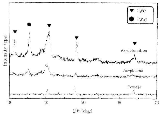
Fig. 5 Traces for WC-NiCr powder and as-sprayed
