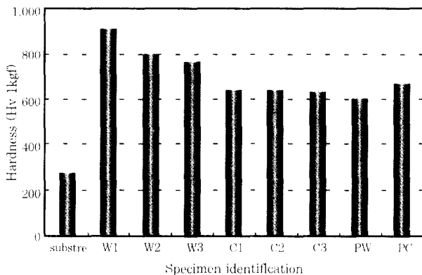
Fig. 4 Variation of micro-hardness with spray condition
