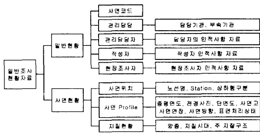
Fig. 7. Schematic diagram for input structure of general data for DB/SLOPE.
