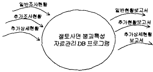
Fig. 4. Data Flow Diagram for DB/SLOPE.
