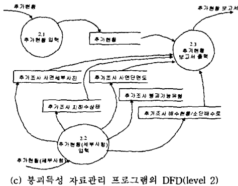
Fig. 5. Data Flow Diagram for DB/SLOPE.
