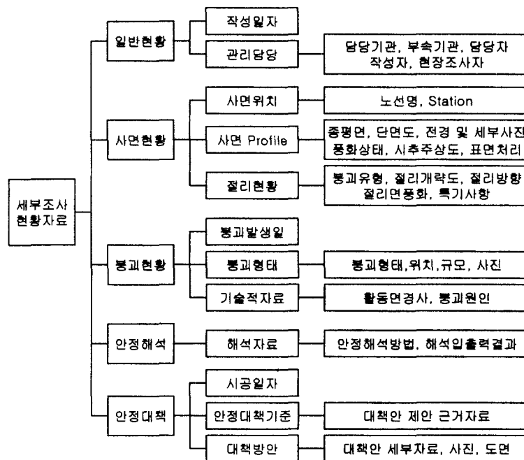
Fig. 8. Schematic diagram for input structure of technical data for DB/SLOPE.
