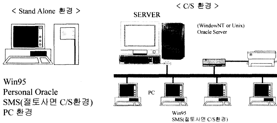
Fig. 2. Stand alone and C/S environment of database system(DB/SLOPE).
