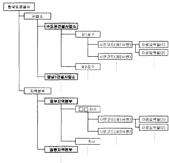
Fig. 10. Flow chart for slope classification and route for data store.
