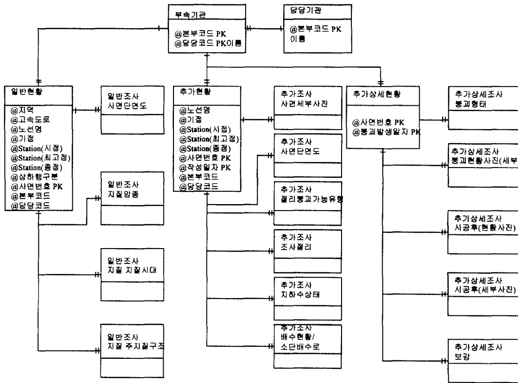
Fig. 3. Entity Relation Diagram for DB/SLOPE.
