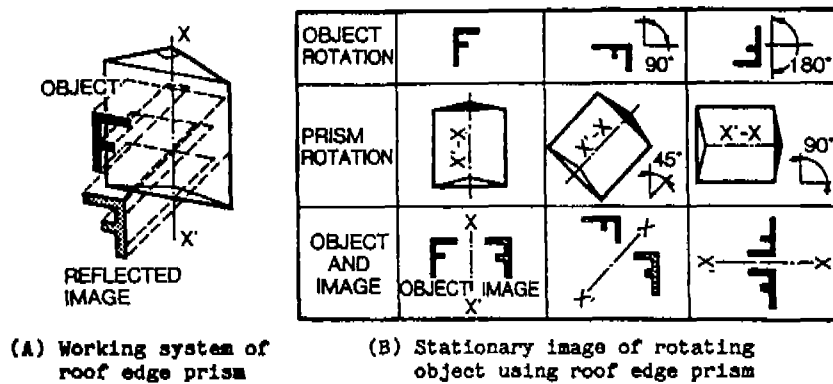
Fig. 3 Optical principle of image de-rotator [Taken from Minami et al.(1992)]
