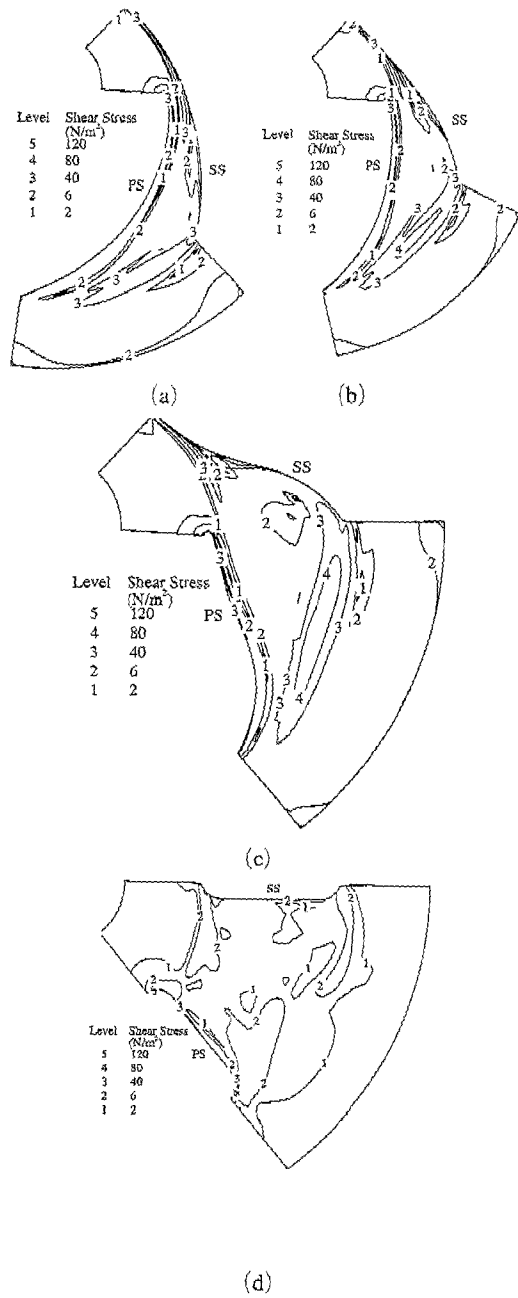
Fig. 7 Shear stress distribution
