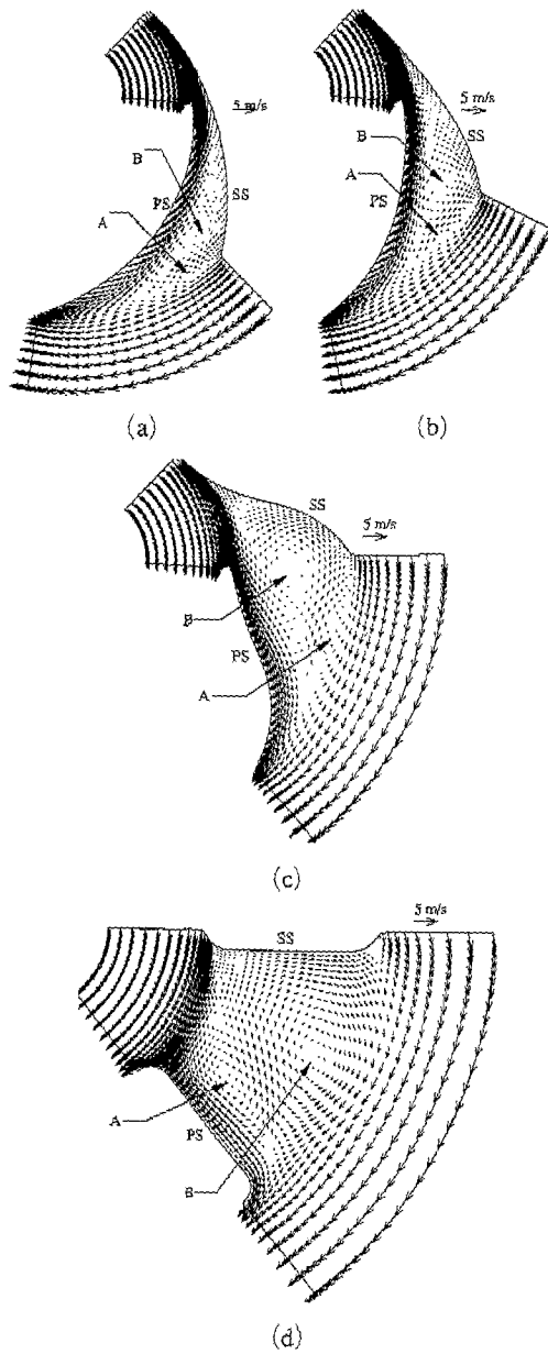
Fig. 6 Velocity distribution
