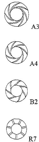
Fig. 2 Impeller Configurations
