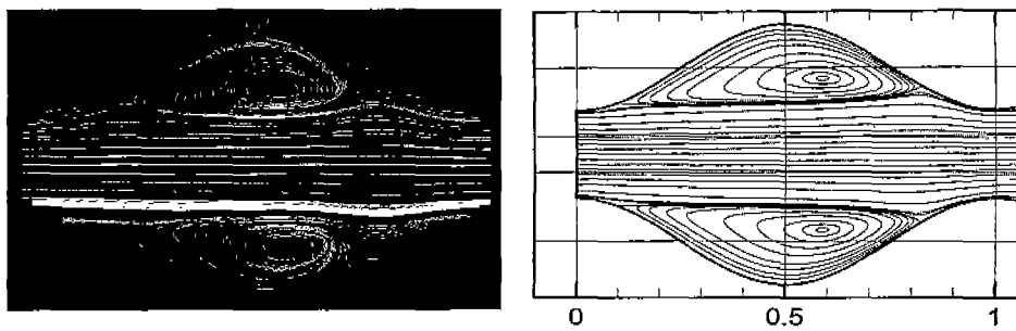
Fig. 4 Mean Streamlines of Numerical Solution (Right) and PIV Result (Left) : Re=500
