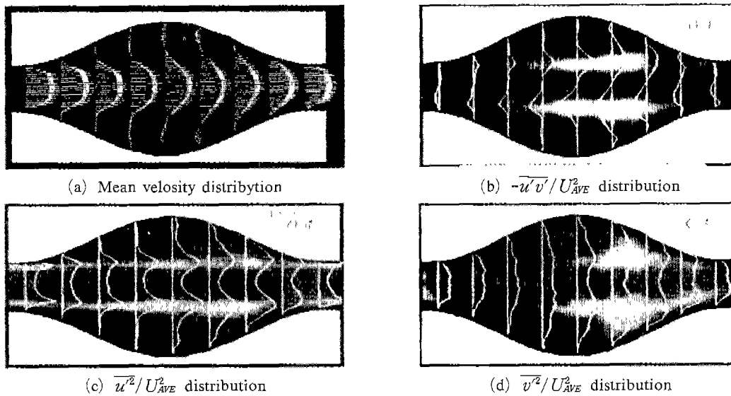
Fig. 8 Mean and Turbulent Intensities for Re = 1000
