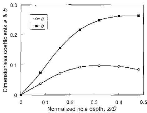
Fig. 4 Dimensionless coefficients, a and b , as functions of hole depth
