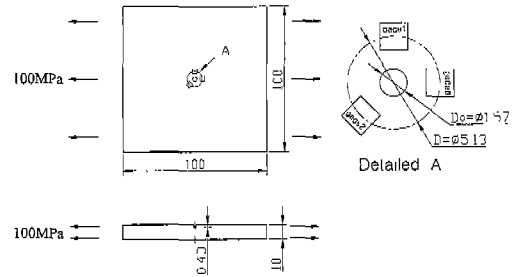
Fig. 5 Model configuration
