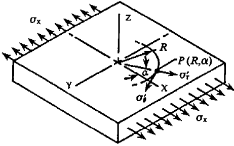
Fig. 1 Stress states at P(R, \alpha) before the hole drilling
