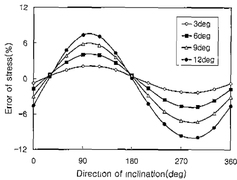
Fig. 8 Error in stress versus the direction of inclination
