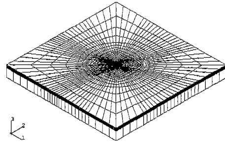
Fig. 6 3-Dimensional finite element model
