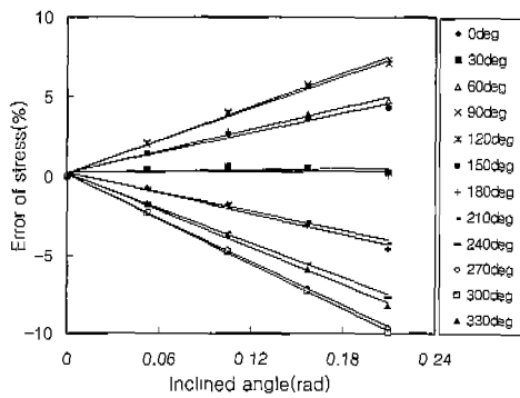
Fig. 9 Error in stress versus inclined angle for various directions of inclination
