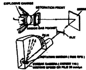
그림 8. Measurement of the detonation front using high-speed photo-graphy, in this case, the curved front in a test charge is swept out over a photographic film at 20,000 m/s by a rotating mirror.
