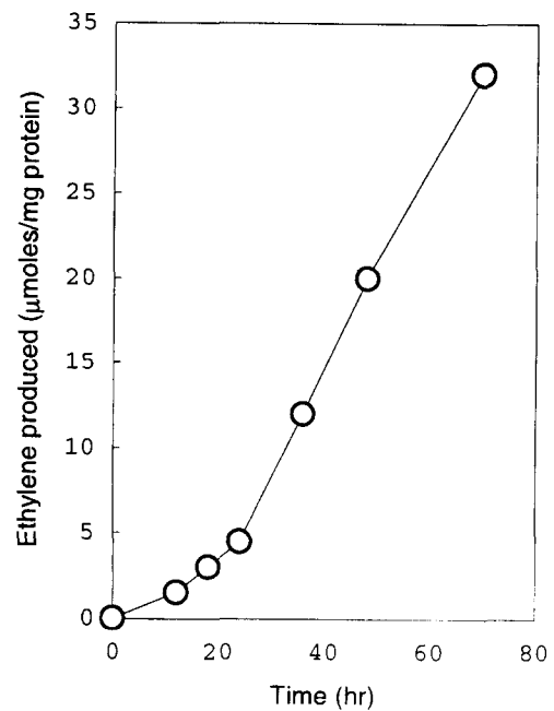
Fig. 1. Acetylene reduction to ethylene by MA547.
