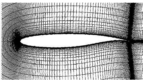
Fig. 2(b) Grid closed-up for DLBA 243 airfoil
