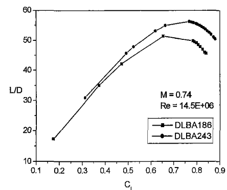
Fig. 11 Lift-to-drag ratio versus lift coefficient
