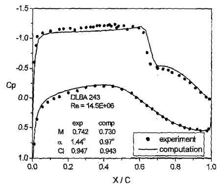
Fig. 4 Measured and computed pressure distributions on DLBA 243 airfoil
