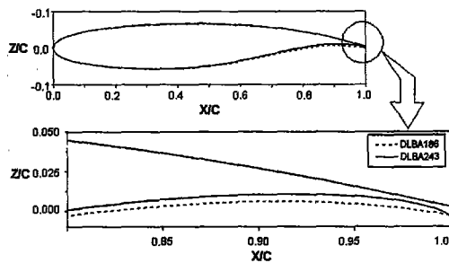
Fig. 1 Geometry of DLBA 186 and DLBA 243 airfoils
