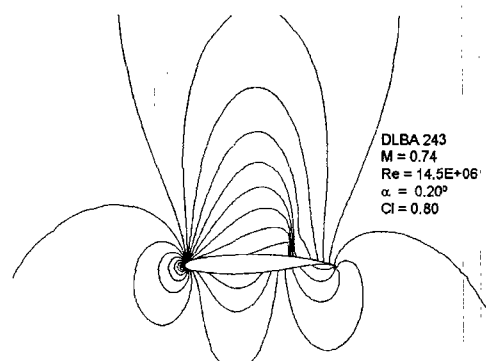
Fig. 7(b) Pressure contours around DLBA 243 airfoil
