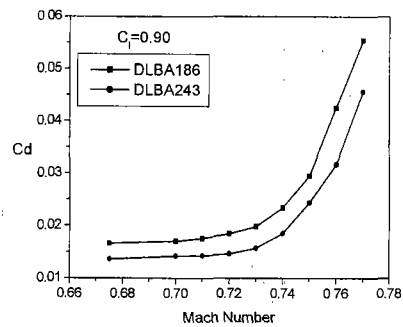
Fig. 13(d) Drag coefficients versus Mach number at a constant lift coefficient of 0.9
