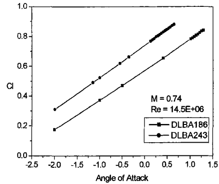
Fig. 9 Lift coefficient versus angle of attack for DLBA 186 and DLBA 243 airfoils
