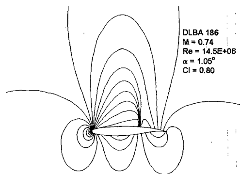
Fig. 7(a) Pressure contours around DLBA 186 airfoil
