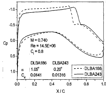
Fig. 6 Pressure distributions on DLBA 186 and DLBA 243 airfoils II
