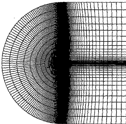
Fig. 2(a) C-Grid system
