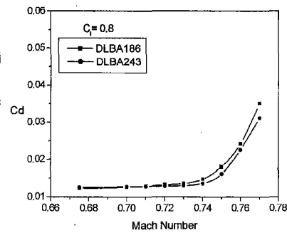
Fig. 13(b) Drag coefficients versus Mach number at a constant lift coefficient of 0.8
