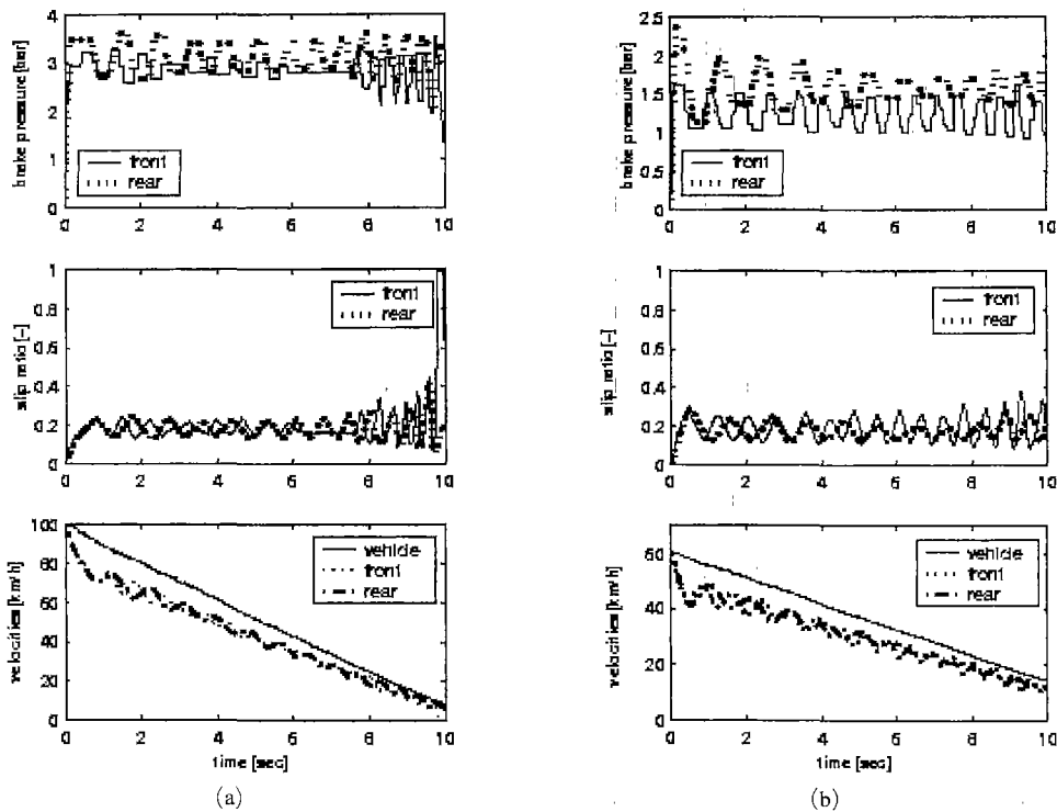
Fig. 8 Vehicle characteristics (a) at higher velocity (100km/h) (b) with lower road friction of \mu=0.15
