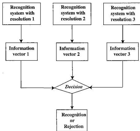
Fig. 3 Architecture of multi-resolution system
