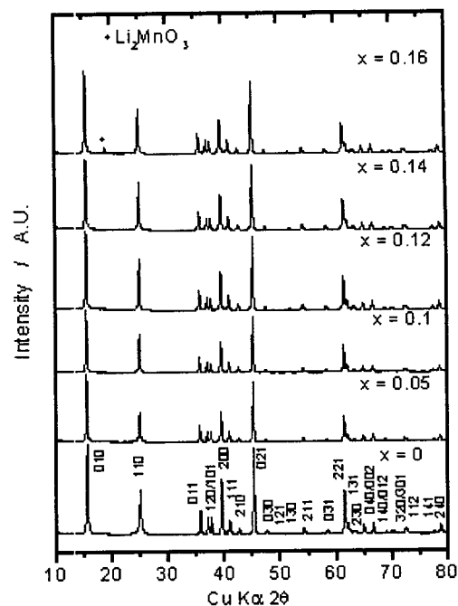
Fig. 1. XRD patterns of Co doped \sigma\text{-LiMnO}_2 as a function of Co doping amount, x in \text{LiCo}_x\text{Mn}_{1-x}\text{O}_2 .
