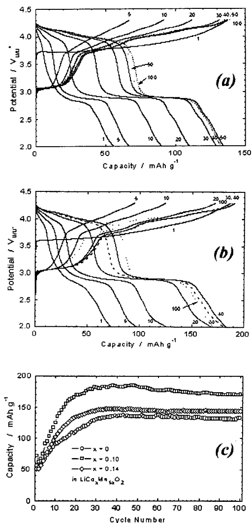
Fig. 2. Charge-discharge profiles of (a) \sigma\text{-LiMnO}_2 , (b) \sigma\text{-LiCo}_{0.1}\text{Mn}_{0.9}\text{O}_2 and (c) their cyclability at 25^\circ\text{C} .
