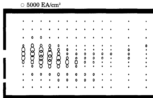
Fig. 14 Particle concentration in Exp.4
