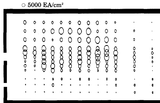
Fig. 15 Particle concentration in Exp.5
