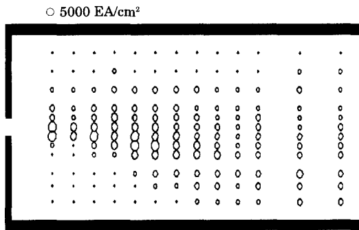
Fig. 11 Particle concentration in Exp.1
