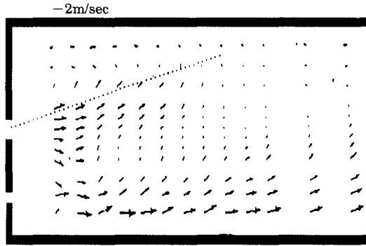
Fig. 9 Particle mean velocity in Exp.5
