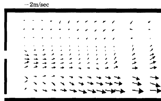
Fig. 7 Particle mean velocity in Exp.3
