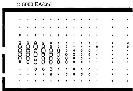
Fig. 12 Particle concentration in Exp.2
