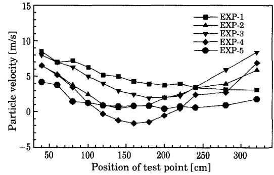
Fig. 10 Comparison of particle velocities on the central axis
