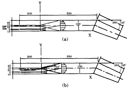
Fig. 2 Coordinate system and section
