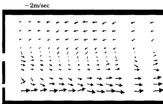
Fig. 6 Particle mean velocity in Exp.2
