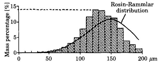
Fig. 3 Particle diameter distribution
