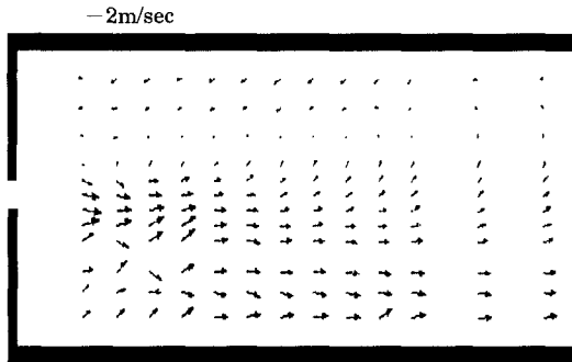
Fig. 5 Particle mean velocity in Exp.1
