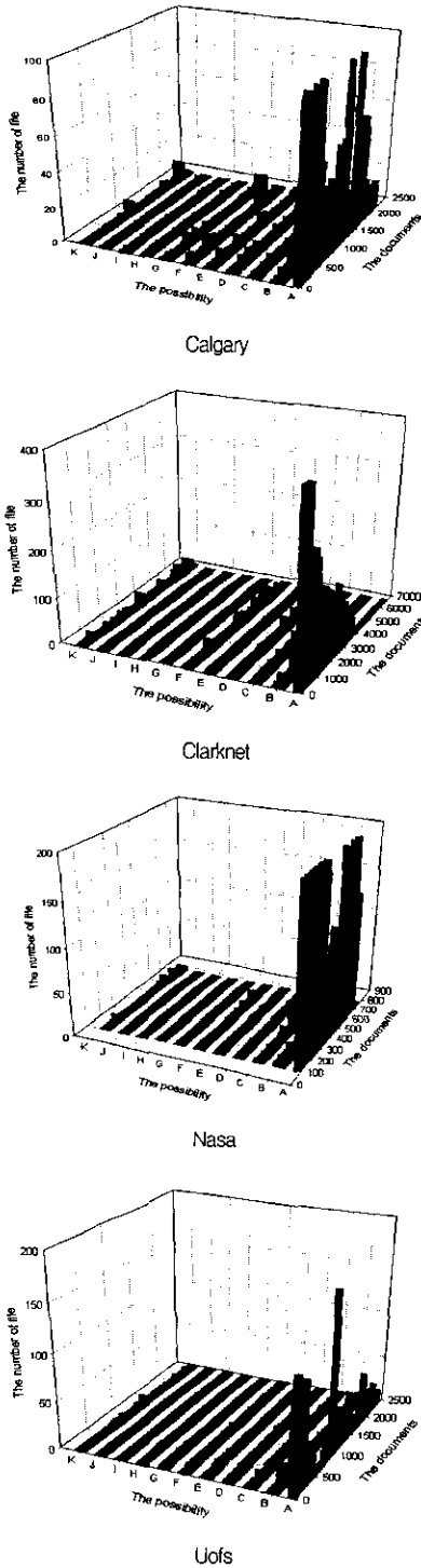
(그림 4) 각 작업부하의 참조적 지역성- A : 0%-9%, B : 10%-19%, C : 20%-29%, D : 30%-39%, E : 40%-49%, F : 50%-59%, G : 60%-69%, H : 70%-79%, I : 80%-89%, J : 90%-99%, K : 100%이상
