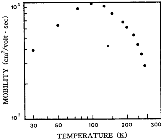
Fig. 11. Temperature dependence of mobility for ZnIn 2 S 4 single crystal thin film.
