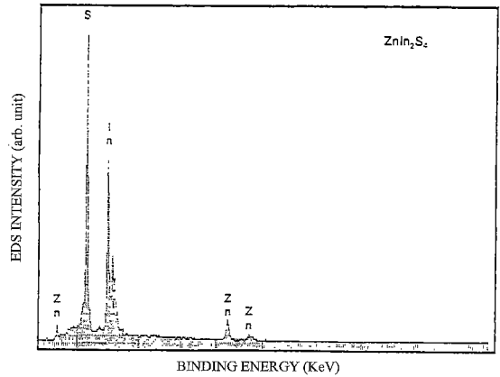
Fig. 9. EDS of ZnIn 2 S 4 single crystal thin film.
