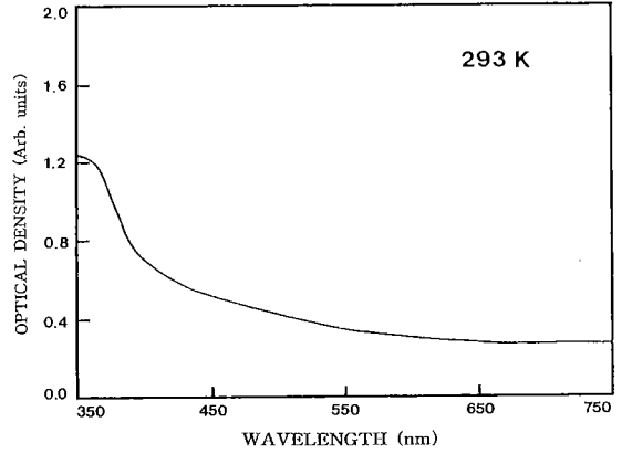
Fig. 12. Optical absorption spectrum of ZnIn 2 S 4 single crystal thin film.
