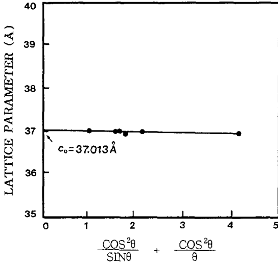
Fig. 5. Lattice constant c_0 of ZnIn 2 S 4 polystal.
