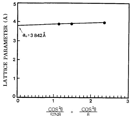
Fig. 4. Lattice constant a_0 of ZnIn_2S_4 polycrystal.
