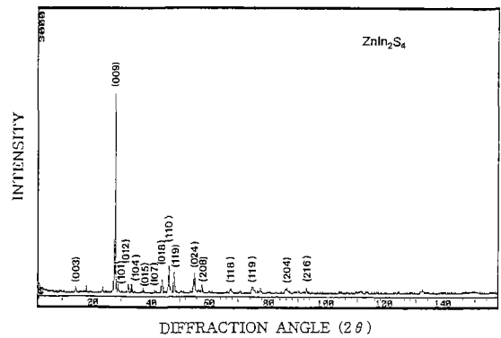
Fig. 3. X-ray diffraction patterns of ZnIn_2S_4 polycrystal.
