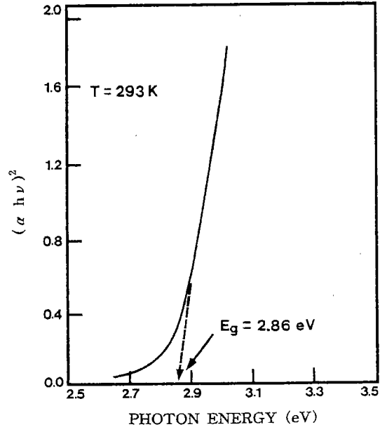
Fig. 13. Plots of (\alpha hv)^2 versus the incident photon energy hv for ZnIn 2 S 4 single crystal thin film.
