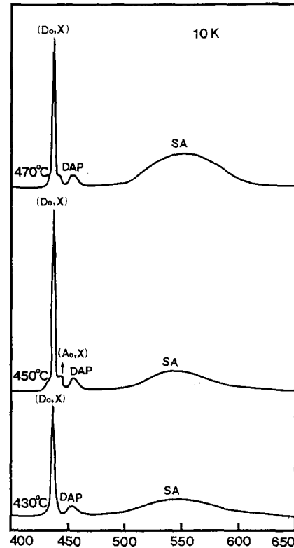
Fig. 6. PL spectrum at 10 °K for various substrate temperatures.
