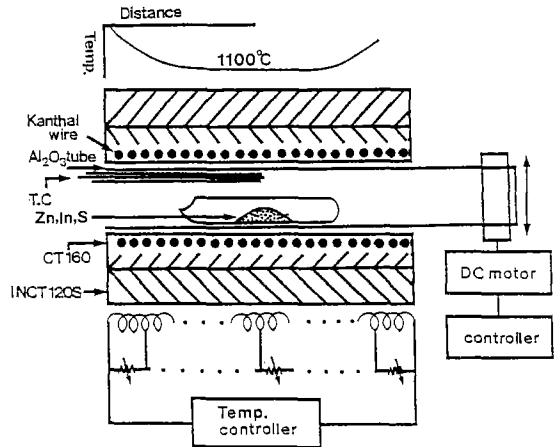
Fig. 1. Horizontal furnace for synthesis of ZnIn 2 S 4 polycrystal.
