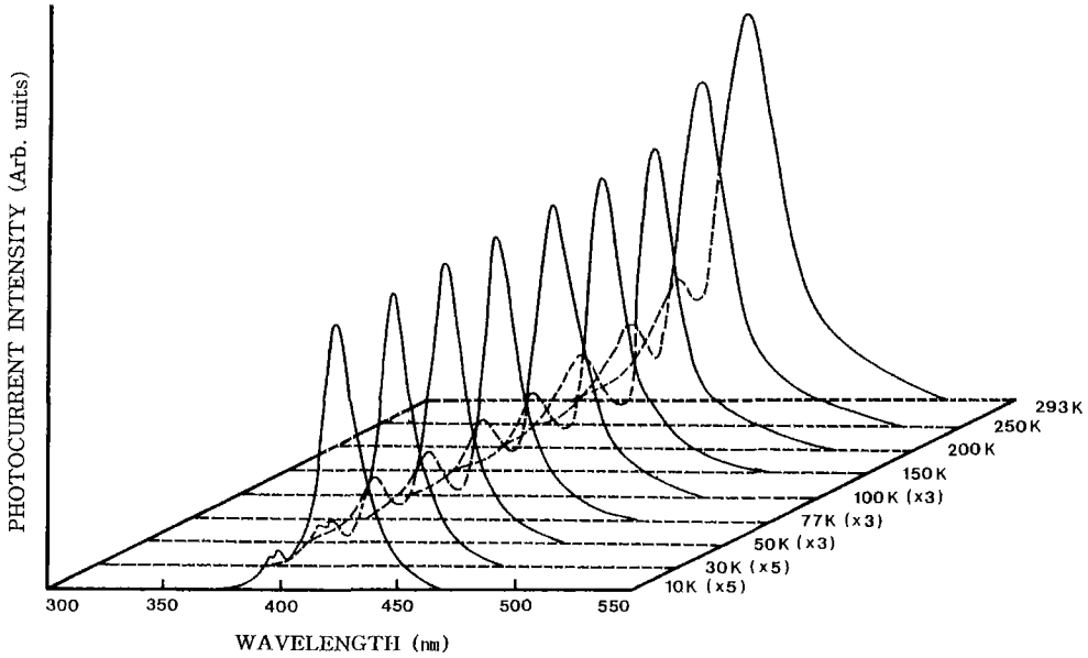
Fig. 14. Photocurrent spectra of ZnIn 2 S 4 single crystal thin film.
