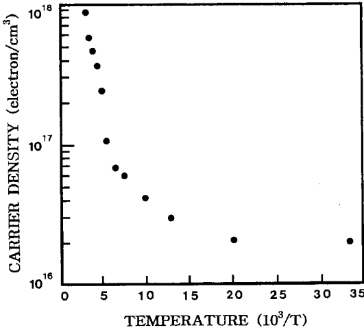
Fig. 10. Temperature dependence of carrier density for ZnIn 2 S 4 single crystal thin film.
