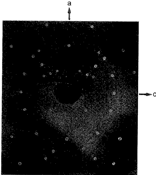
Fig. 8. Back-reflection Laue patterns for the ZnIn 2 S 4 (110) planes.
