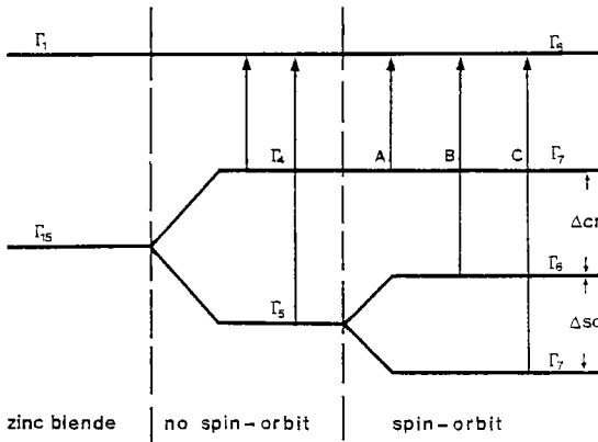
Fig. 15. Fine structure of energy levels of ZnIn 2 S 4 .
