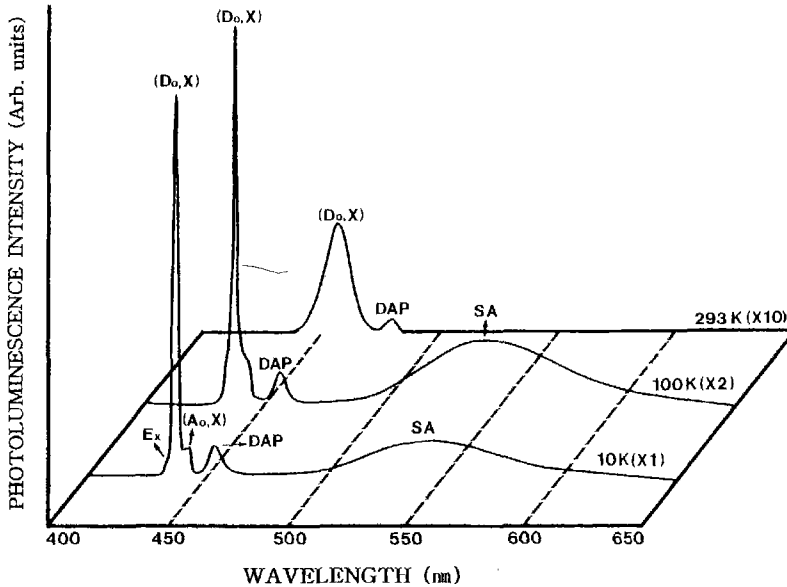
Fig. 16. Photoluminescence spectrum of \text{ZnIn}_2\text{S}_4 single crystal thin film.
