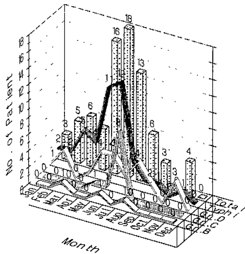
Fig. 1. Detection frequency of Salmonella strains isolated by month in Pusan in 2000.
