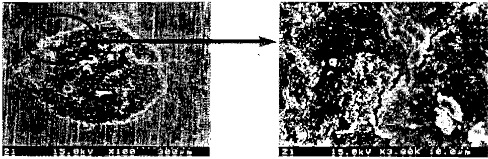
Fig. 8 SEM photograph showing crack generation (Zircaloy-4, 40 \mu\text{m} , 20 N, 1 \times 10^6 cycles)
