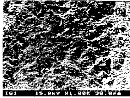
(b) Inconel 600, 300 \mu\text{m} , 20 N, 1 \times 10^5 cycles
