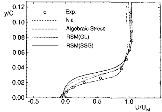
Fig. 3 Mean axial velocity profiles at 87.5 % chord
