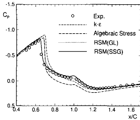
Fig. 2 Pressure coefficients
