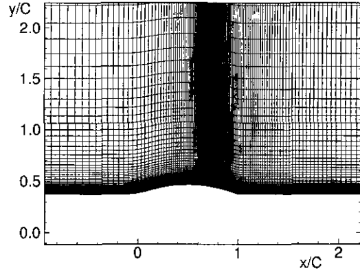
Fig. 1 Grid system
