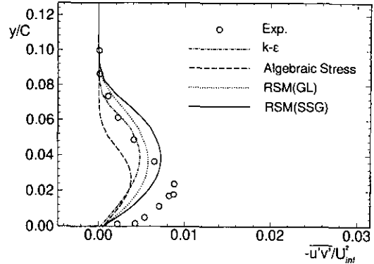
Fig. 8 Turbulent shear stress profiles at 125 % chord
