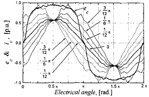
(a) The phase current profiles for producing ripple free torque
