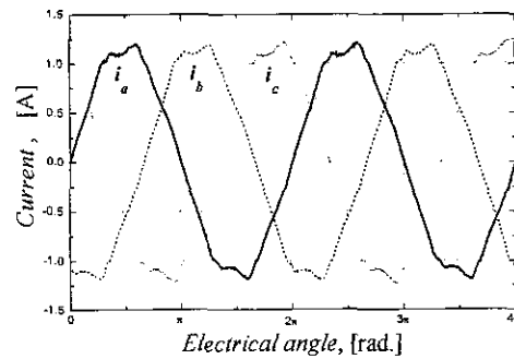
(b) Optimized phase current waveforms for ripple-free torque including cogging torque
