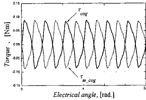
(a) Measure cogging torque \tau_{cog} and mutual torque \tau_{m-cog} for compensating the cogging torque
