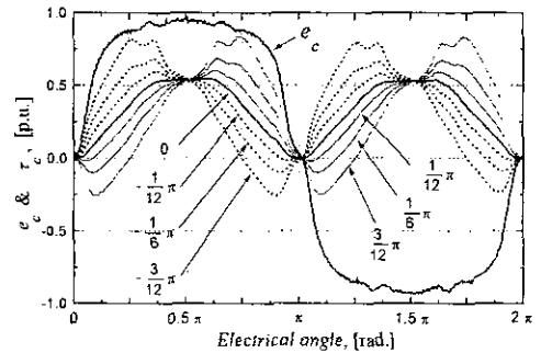
(b) The corresponding phase torque profiles
