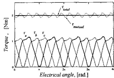
(c) Waveforms of the optimized torque per phase \tau_a, \tau_b, \tau_c , and total mutual torque \tau_{mutual} and resultant developed torque \tau_{atotal} at the motor shaft
