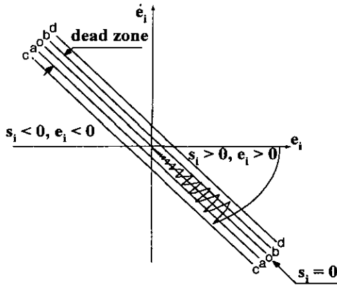
Fig. 2 Phase plane with a pre-determined dead zone around the switching line
