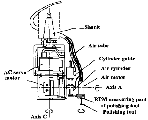
Fig. 1 Polishing robot with two degrees of freedom
