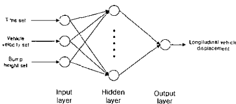
Fig. 12 Neural network for vehicle bump simulation
