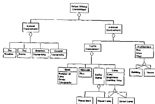
Fig. 5 Class hierarchy of driving environment
