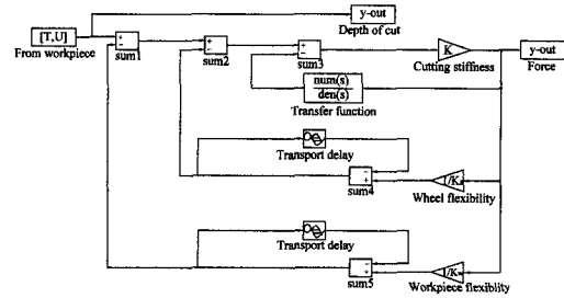
Fig. 3 SIMULAB model of the intermittent grinding process
