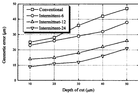
Fig. 8 Geometric error of the conventional and intermittent wheels
