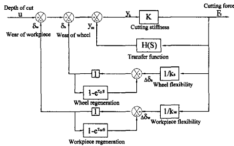
Fig. 2 Representation of a block diagram for estimating the grinding force
