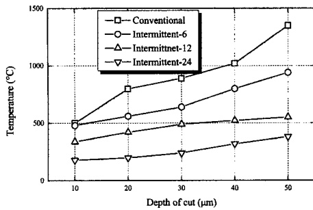
Fig. 7 Grinding temperature of the conventional and intermittent wheels
