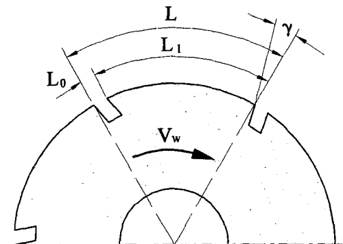
Fig. 1 Schematic drawing of an intermittent grinding wheel
