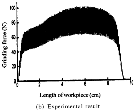
Fig. 4 Grinding forces of the simulation and experimentation
