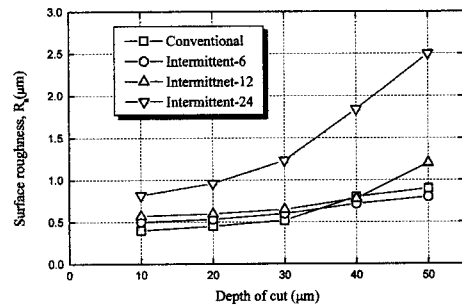
Fig. 6 Surface roughness of the conventional and intermittent wheels
