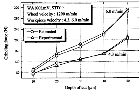
Fig. 5 Result comparison of the simulation and experimentation for grinding force
