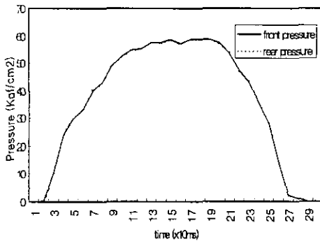
Fig. 29 Experimental brake line pressure result of electronic system with 2351kg at medium level deceleration
