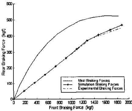
Fig. 35 Electronic system results for 2351kg
