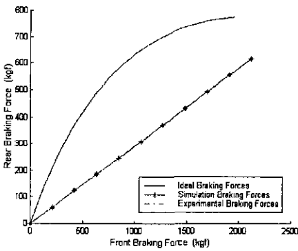
Fig. 36 Electronic system results for 2738kg
