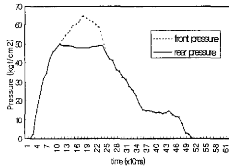
Fig. 26 Experimental brake line pressure result of electronic system with 1840kg at medium level deceleration
