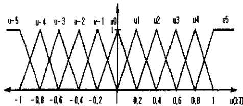
Fig. 16 Membership functions for output universe of discourse
