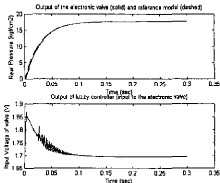
Fig. 24 Simulation results of the direct adaptive fuzzy controller for 2738kg 0.1g
