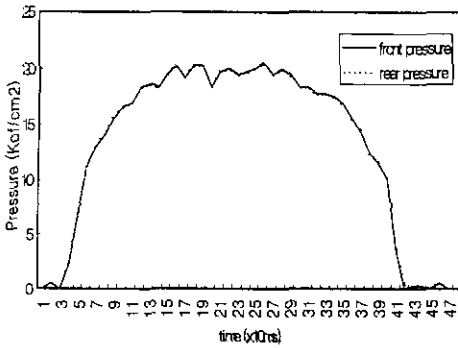
Fig. 28 Experimental brake line pressure result of electronic system with 2351kg at low level deceleration
