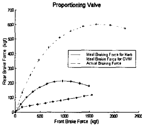
Fig. 4 Braking force of a P.V.
