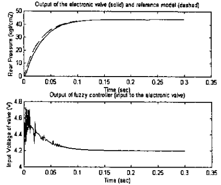
Fig. 21 Simulation results of the direct adaptive fuzzy controller for 1840kg at 0.1g
