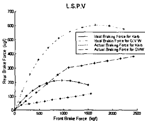
Fig. 6 Braking force of L.S.P.V.
