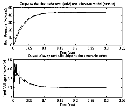
Fig. 22 Simulation results of the direct adaptive fuzzy controller for 1840kg at 1.0g
