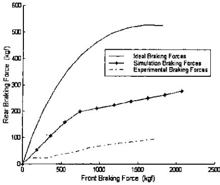
Fig. 19 Mechanical system results for 2351kg
