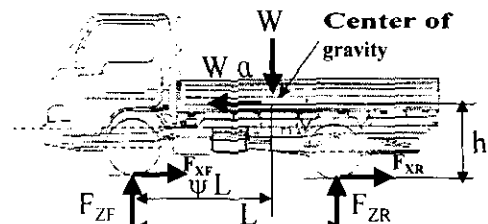
Fig. 1 Dynamic forces acting on a decelerating vehicle
