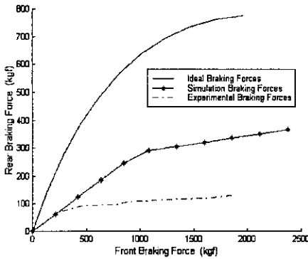
Fig. 20 Mechanical system results for 2738kg
