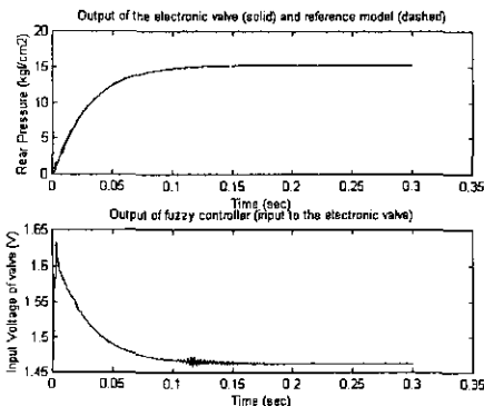
Fig. 23 Simulation results of the direct adaptive fuzzy controller for 2351kg at 0.1g
