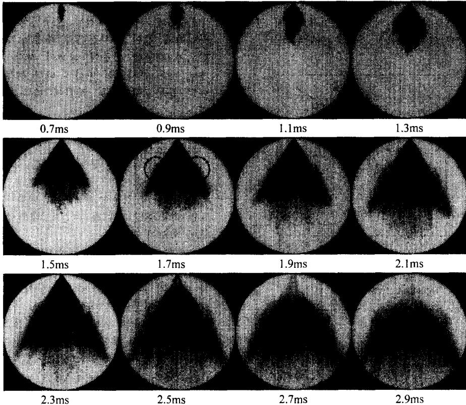
Fig. 9 Time history of GDSI spray phenomena ( P_{inj} = 4.5MPa , T_{inj} = 2.5ms )
