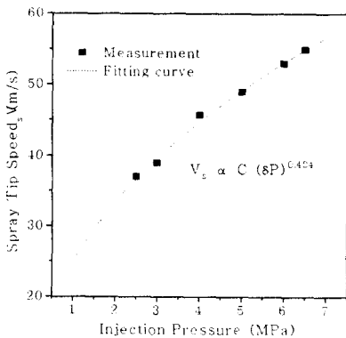
Fig. 13 Relation between injection pressure and spray tip speed
