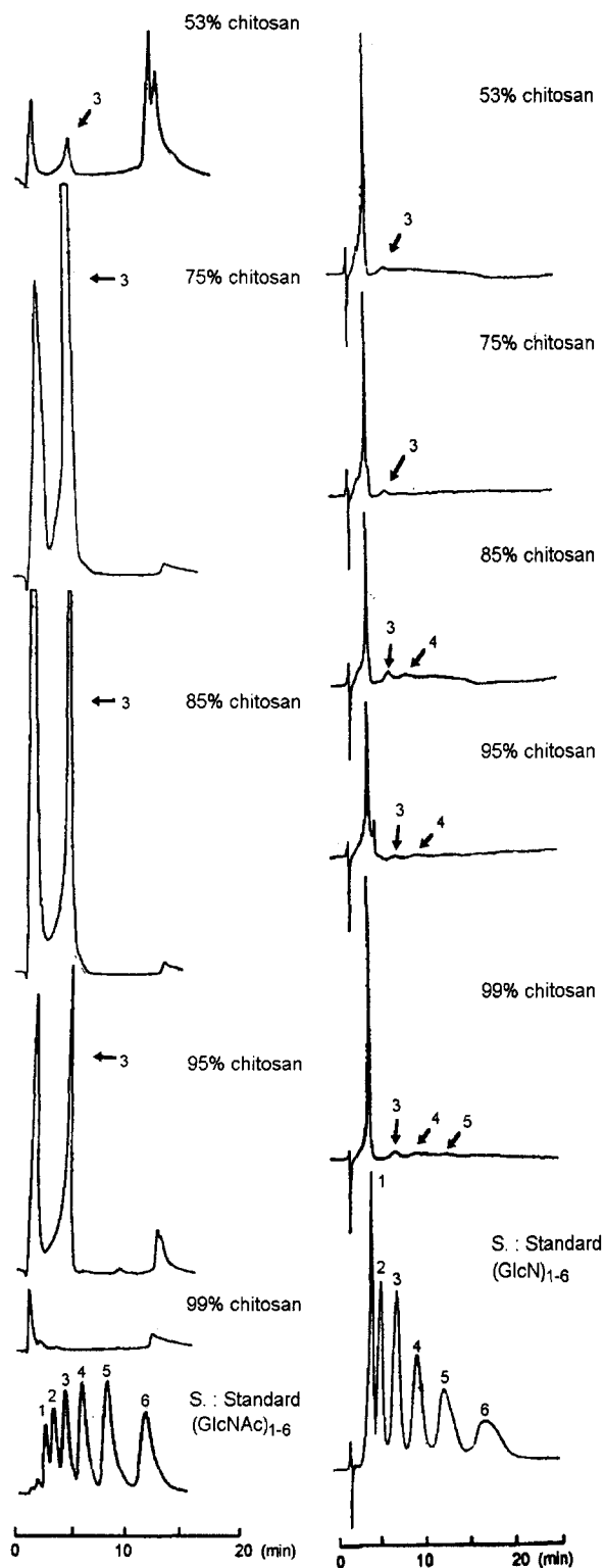
Fig. 5. HPLC chromatograms of chitooligosaccharides produced by enzymatic hydrolysis of various deacetylated chitosans (53-99%) analyzed with UV and RI detectors.
