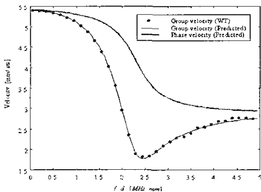
Fig. 11 Measured and predicted group velocity in S_0 mode
