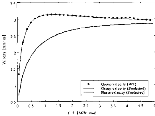
Fig. 9 Measured and predicted group velocity in A_0 mode
