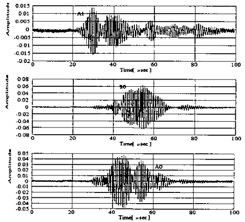
Fig. 7 Typical Lamb wave signal received in Aluminum plate(1 x 1mm slit notch)
