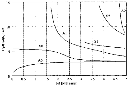
Fig. 1 Dispersion curve for aluminum(phase velocity)
