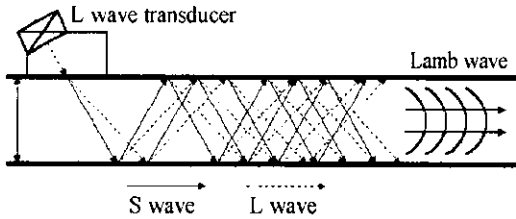
Fig. 5 Oblique incidence method for the generation of guided waves
