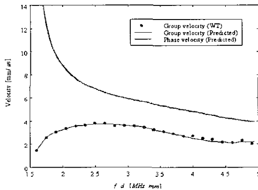
Fig. 10 Measured and predicted group velocity in A_1 mode
