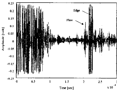
Fig. 6 RF-signal include flaw signal ( A_0 mode)
