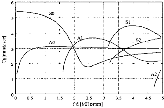
Fig. 2 Dispersion curve for aluminum(group velocity)
