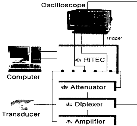
Fig. 4 Schematic diagram of the experimental set-up
