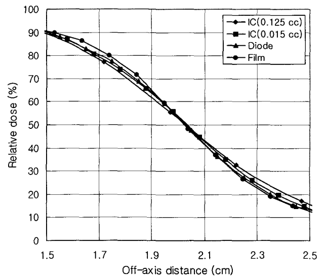
Fig. 7. Penumbra of 4 \times 4 cm field for a 6 MV x-ray measured with four different kind of detectors which are ionization chamber (IC) of 5.5 mm (0.125 cc) and 2.0 mm (0.015 cc) inner diameter, diode detector of 2.5 mm inner diameter, and a film.
