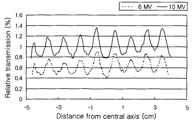
Fig. 6. Interleaf and midleaf transmissions measured at d_{max} in solid water phantom with radiographic film for 6 and 10 MV X-rays. The transmission is the ratio of the MLC blocked field to the 10 \times 10 cm^2 open field.
