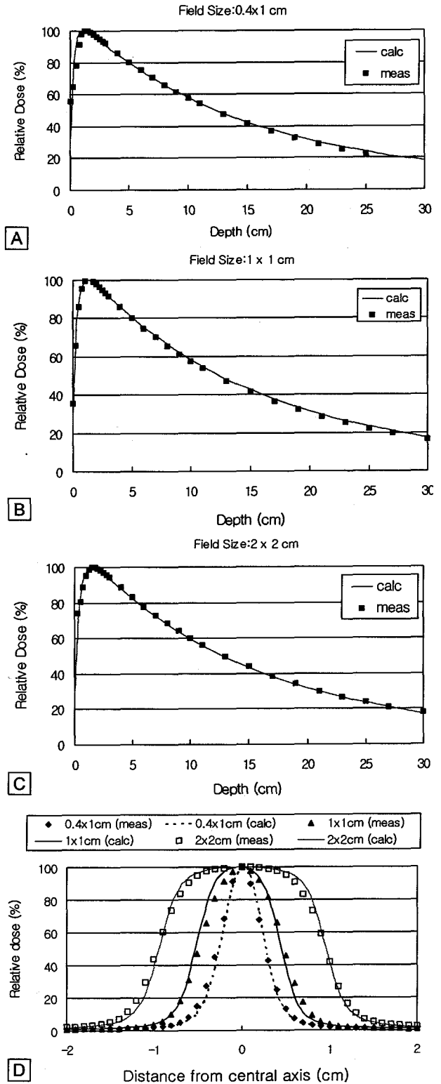
Fig. 9. Calculated and measured small field depth dose profiles for a 6 MV x-ray. depth dose profiles of (A) 0.4×1 cm field size, (B) 1×1 cm field size, (C) 2×2 cm field size, and (D) off-axis profiles.
