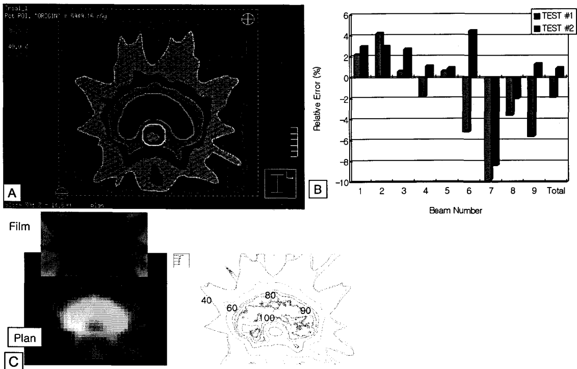
Fig. 10. Test plan of C-shaped target with 9-field intensity modulated beams arranged by 40 degrees equi-angular steps, i.e. 0, 40, 80, 120, 160, 200, 240, 280, and 320 degrees (A). (B) Isocenter dose verification with PinPoint micro ionization chamber in 30×30 cm 2 solid-water phantom. The beam number 6 and 7 are corresponding to the gantry angles of 160, 200 degrees respectively. These two beam produced very steep dose gradient across the isocenter and relatively large discrepancies for these two beams came from chamber positioning uncertainty. The relative error is the ratio of a planed dose to measured dose. (C) Comparison of dose distribution on plane of isocenter between calculation and EC-L film measurement
