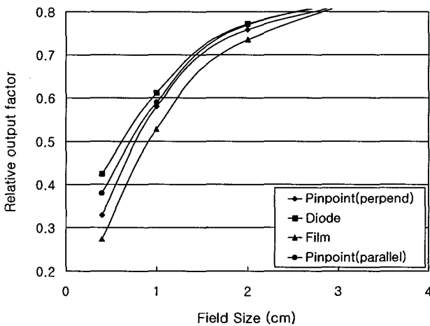
Fig. 8. Output factor for 6 MV x-rays measured with various detectors, PinPoint ionization chamber, diode detector, and film. The ionization chamber and the film underestimate the outputs for small fields (see text for details).
