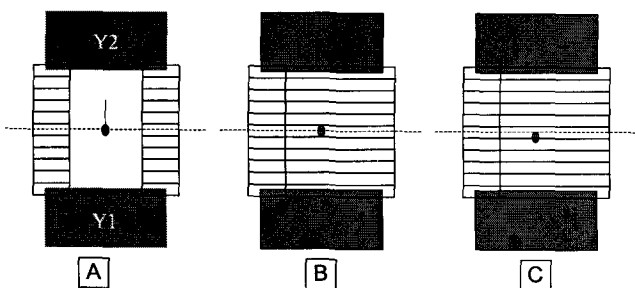
Fig. 5. Schematic diagram of detector and collimator positions for measuring interleaf and midleaf transmissions. The midleaf transmission was measured at the beam central axis while the junction between the opposed leaves was placed 5cm off axis to avoid leakage between the leaf ends (B), the interleaf leakage was measured at the junction between the central leaf and the next leaf (C).
