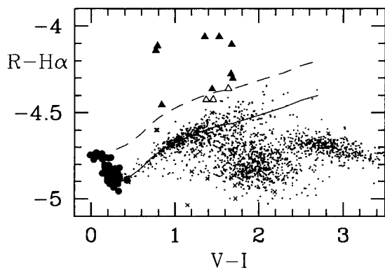
Fig. 5. — The R - H\alpha vs. V - I diagram. The solid line represents the MS relation adopted from Sung et al. (1997), but shifted by E(V - I) = 0^m.13 and the dashed line shows the selection limit of H\alpha emission stars. Symbols are the same as in Fig. 3.
