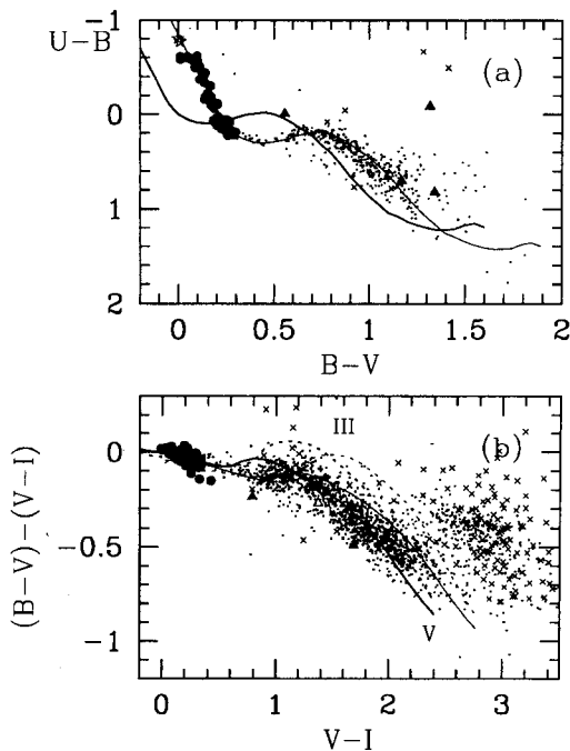
Fig. 3. — Color-color diagrams. The ZAMS relation for main sequence stars (V: solid line) and that for giant stars (III: dotted line) brighter than V = 18^m are shown. Thick lines are for the same relations but reddened by E(B - V) = 0.29 . The symbols represent: filled circles – bright members, dots – non-member stars, small crosses – stars with poor photometric quality ( \epsilon \geq 0.1 mag), stars – data from photoelectric photometry of previous investigators, filled triangles – PMS stars, and open triangles – PMS candidates.
