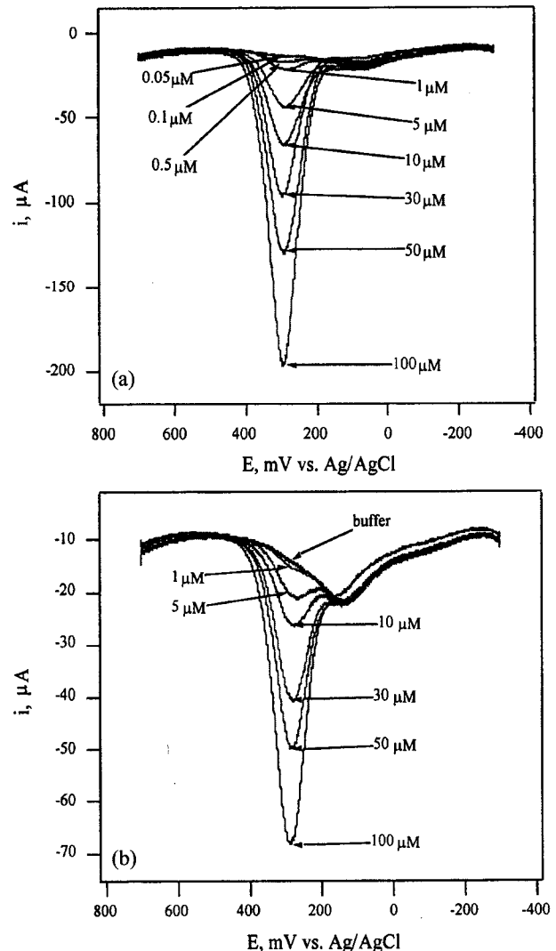
Fig. 3. Square-wave voltammograms for dopamine in the presence of 0.2 mM ascorbic acid at the (a) NHS-modified and (b) unmodified carbon paste electrodes. (amplitude : 70 mV; frequency : 100 Hz ; buffer: 0.1 M pH 4.0 PBS with 140 mM NaCl.)
