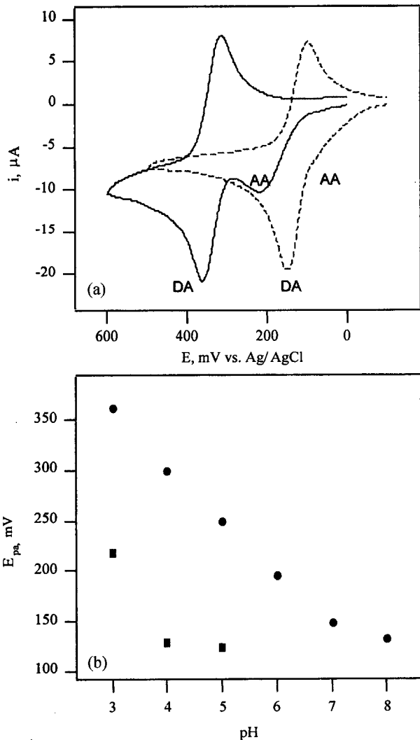
Fig. 2. The effect of pH on the E_{pa} values of dopamine and ascorbic acid: (a) CV for the 1 mM dopamine + 1 mM ascorbic solution at two different pH, 3 (—) and 7 (---); and (b) variation of the E_{pa} values as a function of pH (● dopamine ■ ascorbic acid); scan rate 50 mV/s in a 0.1 M PBS with 140 mM NaCl.
