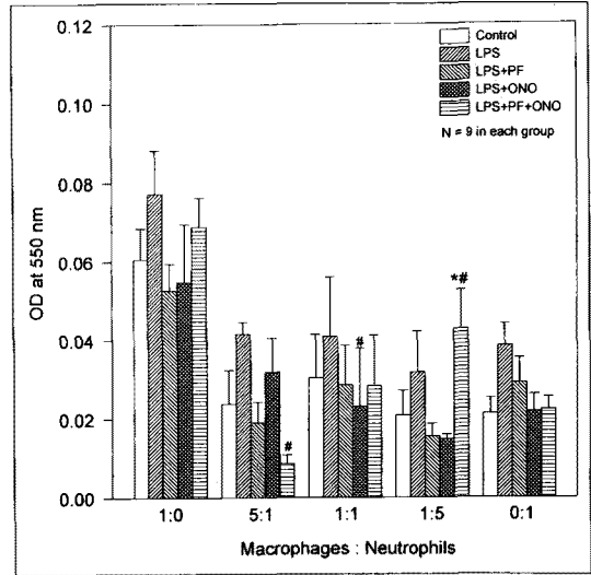
Fig. 1. Effects of pentoxifylline (PF) and neutrophil elastase inhibitor (ONO) on LPS-induced superoxide anion productions from rat alveolar macrophages and/or peripheral neutrophils * P <0.05 compared to the control group, # P <0.05 compared to the LPS group.
