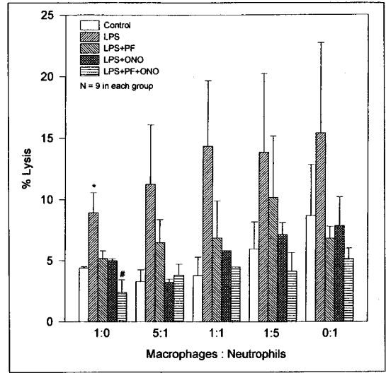
Fig. 3. Effects of pentoxifylline (PF) and neutrophil elastase inhibitor (ONO) on LPS-induced IP2-E4 cell injury by rat alveolar macrophages and peripheral neutrophils * P < 0.05 compared to the control group, # P < 0.05 compared to the LPS group.
