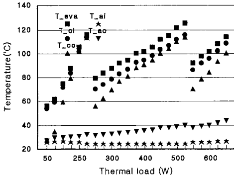
Fig. 10 System temperature variation with thermal load for three layers of 60 mesh screen
