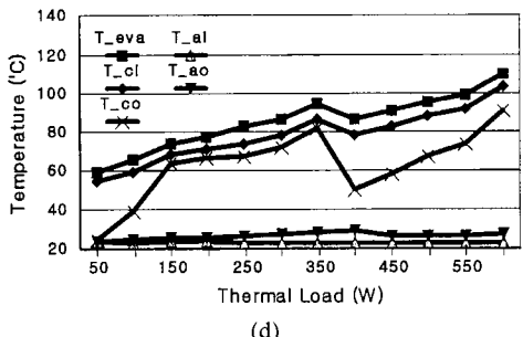
Fig. 4 System temperature variations with thermal load for bare evaporator plate cases. (a) 20% charge(1 condenser open) (b) 30% charge(1 condenser open) (c) 20% charge (2 condensers open) (d) 20% charge(3 condensers open)
