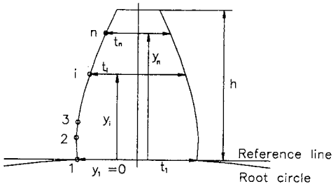
Fig. 1 Measurement of tooth heights and thicknesses
