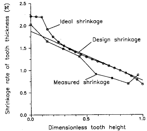
Fig. 4 Variation of shrinkage rate with dimensionless tooth height in the Cavity U
