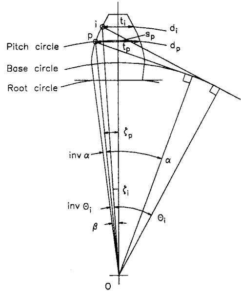
Fig. 2 Tooth geometry
