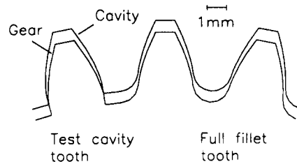
Fig. 5 Teeth of the cavity and molded gear
