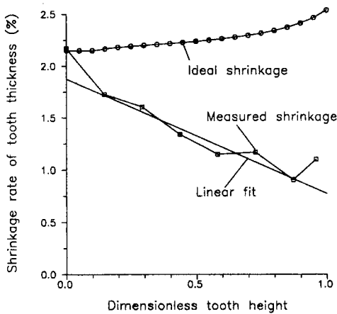
Fig. 3 Variation of shrinkage rate with dimensionless tooth height in the test cavity
