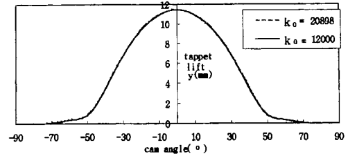
Fig. 7 Equivalent tappet lift (intake)
