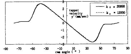
Fig. 8 Equivalent tappet velocity (intake)
