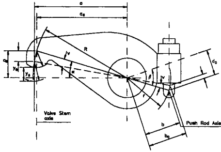
Fig. 2 Geometry of center-pivot type rocker arm
