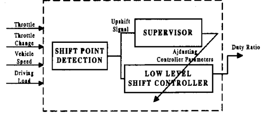
Fig. 6 Shift controller architecture
