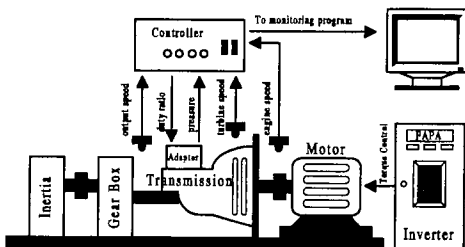
Fig. 10 Experimental apparatus
