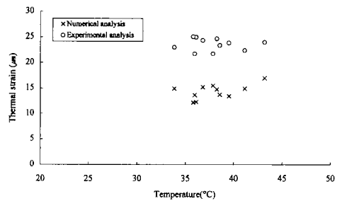
Fig. 7 Thermal strain ( \varepsilon_y ) vs. temperature for [0/90]_{8S}
