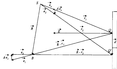
Fig. 1 Relationship between the displacement vector of surface point and phase difference
