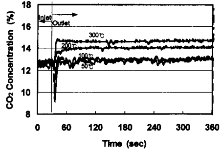
Fig. 4 CO 2 concentration vs. time for various adsorber temperatures
