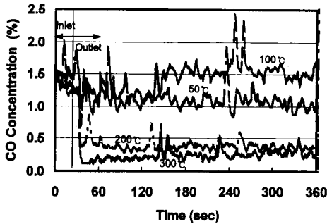
Fig. 3 CO concentration vs. time for various adsorber temperatures
