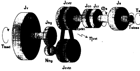
Fig. 3 CVT Powertain model
