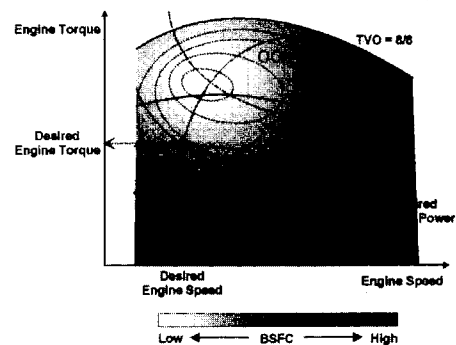
Fig. 1 Engine characteristic curves and OOL
