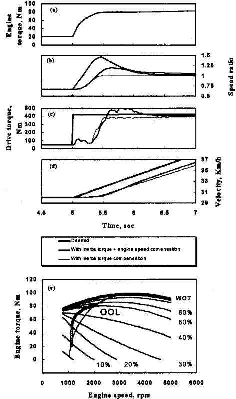
Fig. 6 Response for engine speed compensation for CVT response lag
