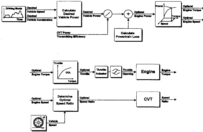
Fig. 2 Block diagram of engine-CVT integrated control algorithm
