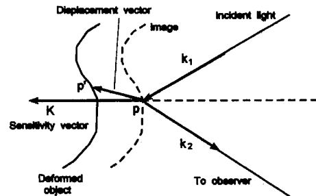
Fig. 2 Vector diagram showing sensitivity to displacement in ESPI
