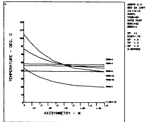
Fig. 5 Temperature rise graph of specimen center after heating and cooling
