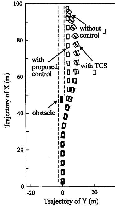
Fig. 7 Vehicle trajectory for lane change maneuver
