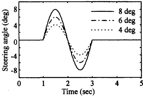
Fig. 2 Different steering angle inputs
