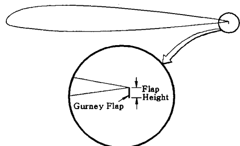
Fig. 1 Gurney flap
