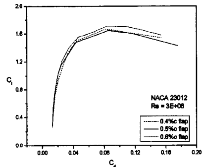
Fig. 13 Drag polars for Gurney flap heights of 0.4c, 0.5c, 0.6c
