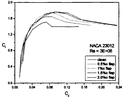
Fig. 10 Drag polars for various Gurney flap heights
