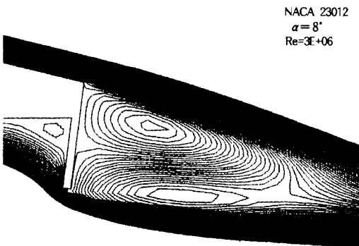
Fig. 17(a) Streamline pattern around 0.6%c height Gurney flap
