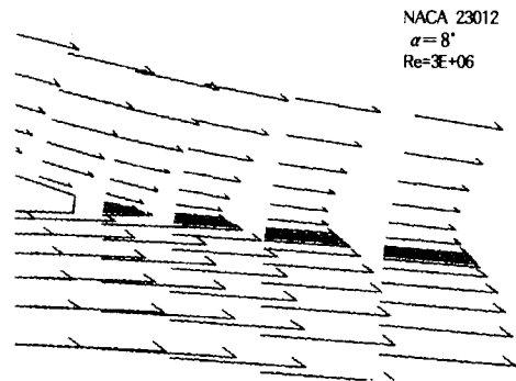
Fig. 16(b) Velocity vector field of clean airfoil
