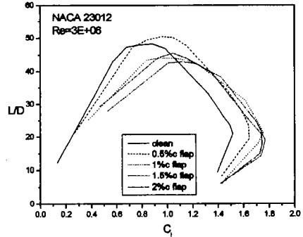
Fig. 12 Lift-to-drag ratio versus lift coefficient for various Gurney flap heights
