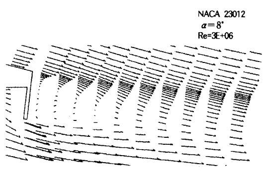
Fig. 17(b) Velocity vector field around 0.6%c height Gurney flap
