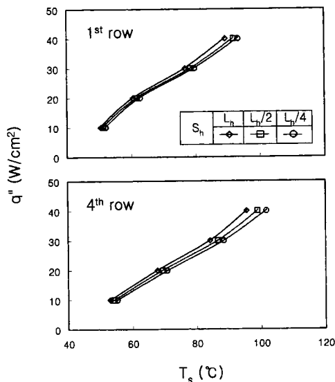
Fig. 4 Removable heat flux for 7.5 % paraffin slurry with respect to the chip surface temperature ( Re_{Dh} = 16,000 )
