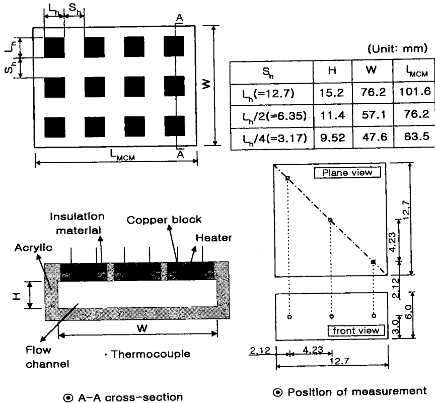
Fig. 2 Details of the present test section
