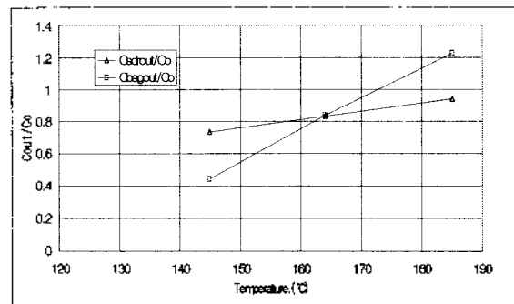
Fig. 5. Effect of SDR temperature on o-DCB removal Experimental condition : gas flow = 3Nm 3 /min, o-DCB = 60mg/Nm 3 , lime = 1767mg/Nm 3 , activated carbon = 600mg/Nm 3 , atomizer r.p.m = 16000
