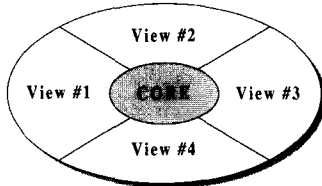
(그림 1) MOVI(Managed Object View Interface)
