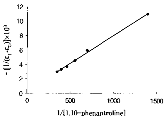
Fig. 6. Plot of 1/(\epsilon_T - \epsilon_0) vs. 1/[1,10\text{-phenanthroline}] in reaction of \text{Sm}^{3+} complex with 1,10\text{-phenanthroline} .
