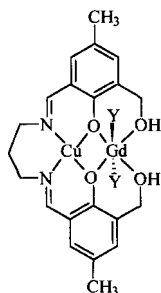
[CuGd(H 2 L[B])(NO 3 ) 2 ](NO 3 )·2CH 3 OH (Y = NO 3 - , bidentate O donor ligand)
