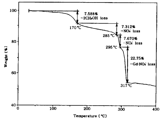
Fig. 1. The thermogravimetric curve of the [\text{CuGd}(\text{H}_2\text{L[B]})(\text{NO}_3)_2(\text{NO}_3)_2 \cdot 2\text{CH}_3\text{OH}] run in nitrogen atmosphere and heating rate 20^\circ\text{C}/\text{min} .
