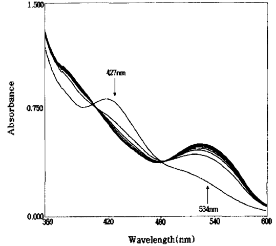
Fig. 4. Spectral changes upon addition of oxalic acid to [Dy([20]DOTA)(NO 3 )(CH 3 OH)] 2+ in methanol at \mu=0.1\text{M NaClO}_4 .
