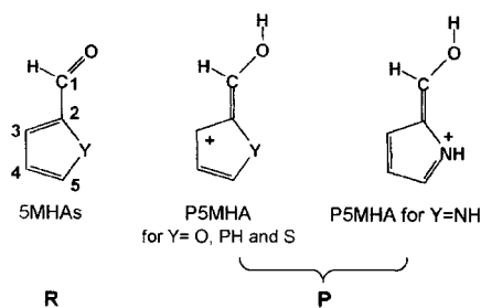
Figure 1. Optimal localized natural Lewis structures for 5MIAs ( R ) and P5MIAs ( P ).
