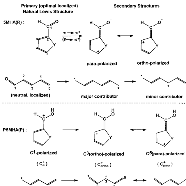
Figure 3. Primary and Secondary Natural Lewis Structures of 5MIAs ( R ) and their protonated forms, P5MIAs ( P ).
