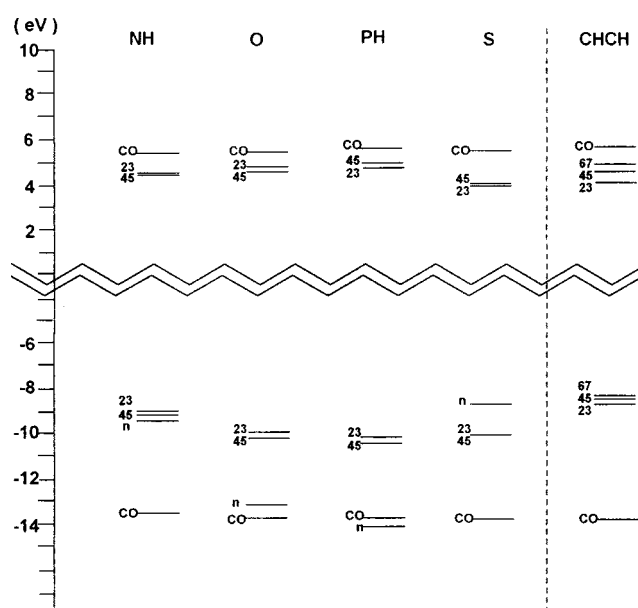
Figure 2. Frontier NBO levels (MP2/6-31G*). The lower half represents bonding orbitals, n, \pi_{CO} , \pi_{23} , \pi_{45} and \pi_{\sigma^*} , and the upper half represents antibonding orbitals, \pi_{CO}^* , \pi_{23}^* , \pi_{45}^* and \pi_{\sigma^*}^* . The n level is the highest for Y = S, whereas the energy gaps, \Delta\epsilon = \epsilon_{\pi^*} - \epsilon_{\pi} , are the narrowest with Y = NH among the 5MIAs.
