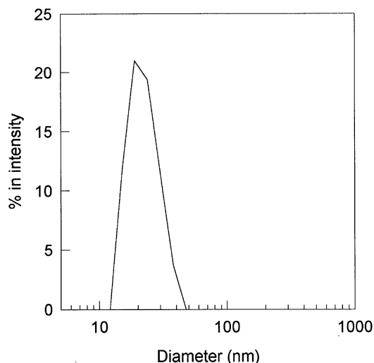
Figure 2. Particle size distribution of GEG polymeric micelles prepared from DMF as the initial solvent.
