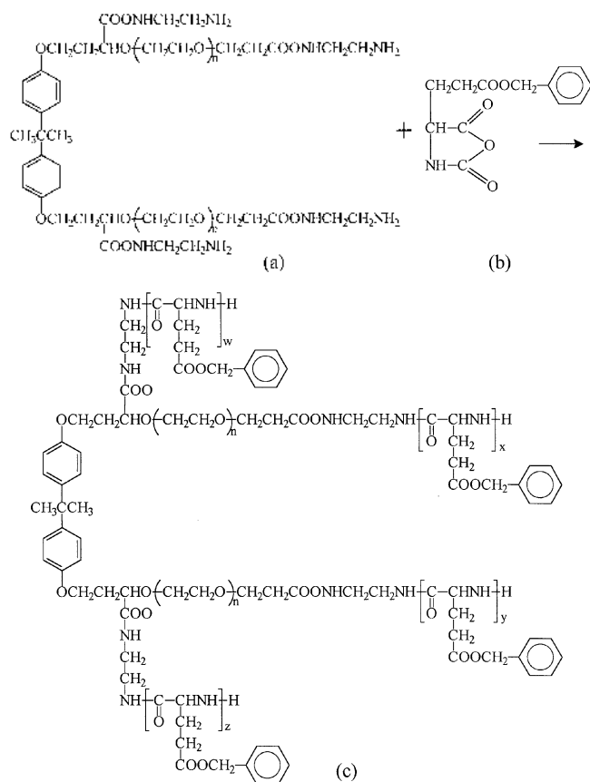
Figure 1. Synthesis scheme of GEG multiblock copolymer.
