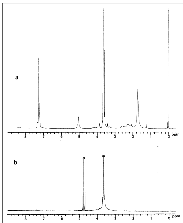
Figure 6. ^1\text{H} NMR spectroscopy of GEG polymeric micelles in \text{CDCl}_3 (a) and \text{D}_2\text{O} (b).
