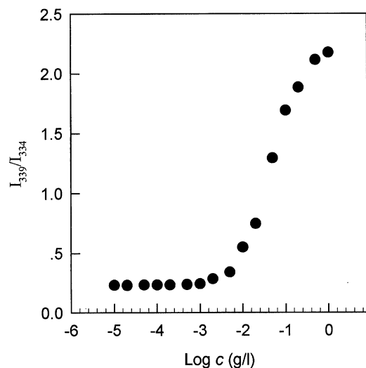
Figure 5. Plot of the intensity ratio I_{339}/I_{334} from pyrene excitation spectra versus \log c for block copolymers against concentration of GEG in distilled water.
