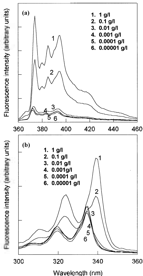
Figure 4. Fluorescence spectra of pyrene ( 6 \times 10^{-7} M)/GEG against concentration of GEG in distilled water (excitation wavelength: 339.0 nm) (a) and excitation spectra of pyrene/GEG against concentration of GEG in distilled water (Emission wavelength: 390.0 nm) (b).
