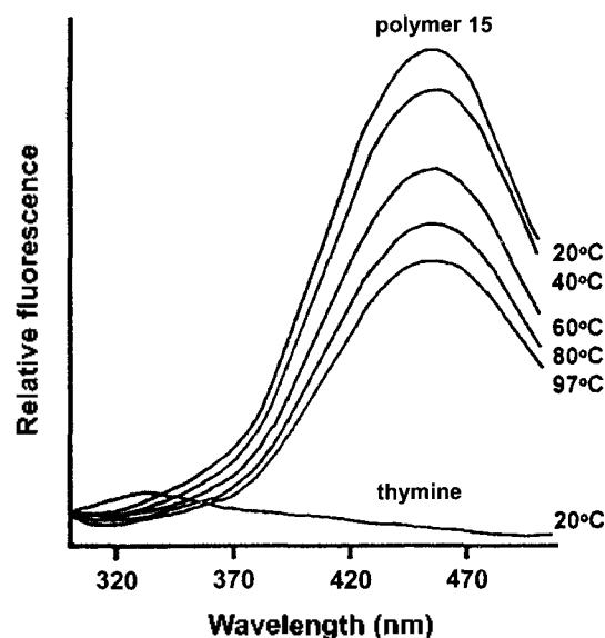
Figure 3. Fluorescence emission spectra of thymine and polymer 15 in \text{H}_2\text{O} at different temperatures after excitation at 250 \text{ nm} .
