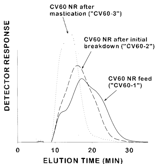
Figure 3. ThFFF fractograms of CV60 NR collected at three different stages of an anaerobic mastication process with the low molecular weight resin peak removed.
