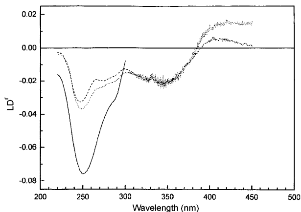
Figure 6. LD' spectrum of the \Delta -(dashed curve) and \Lambda -(dotted curve) enantiomers of [\text{Ru}(\text{phen})_2\text{DPPZ}]^{2+} complexes bound to \text{CGC}^+ triplex. Solid curve denotes the LD' spectrum of metal complex free \text{CGC}^+ triplex. The samples are the same as in Figure 4.
