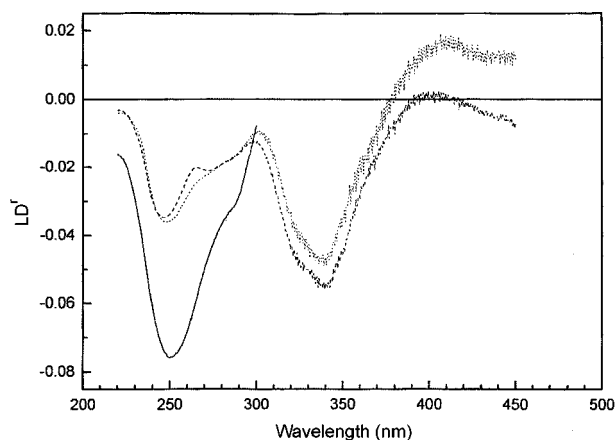
Figure 7. LD' spectrum of the \Delta -(dashed curve) and \Lambda -(dotted curve) enantiomers of [\text{Ru}(\text{phen})_2\text{BDPPZ}]^{2+} complexes bound to \text{CGC}^+ triplex. Solid curve denotes the LD' spectrum of metal complex free \text{CGC}^+ triplex. The samples are the same as in Figure 5.
