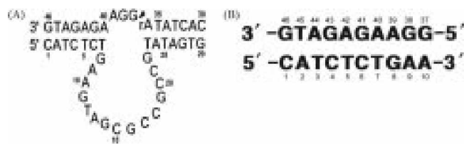
Figure 1. (A) Secondary structure of the complex between the DNAzyme (29 mer) and substrate (17 mer). The substrate contains a single adenosine ribonucleotide, flanked by deoxyribonucleotides. (B) DNA sequence contexts of the left stem of the complex.
