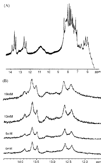
Figure 2. (A) ^1\text{H} NMR spectra for the DNAzyme-substrate complex in \text{H}_2\text{O} buffer solution containing 10 mM sodium phosphate (pH 7.0) and 100 mM NaCl. (B) \text{Mg}^{2+} -dependence of the imino proton resonances of the ^1\text{H} NMR spectra for the complex in \text{H}_2\text{O} buffer solution. The \text{Mg}^{2+} concentrations are shown on the left.
