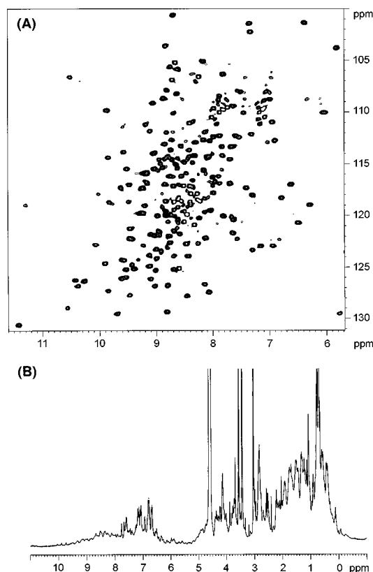
Figure 3. NMR spectra of the ^{15}\text{N} -labeled amidase domain of GSP synthetase/amidase. ^1\text{H} - ^{15}\text{N} HSQC spectrum (A) and 1D NMR spectrum (B) were acquired in 90% \text{H}_2\text{O}/10\%\text{D}_2\text{O} with 50 mM NaPi, pH 6.5, 300 mM NaCl, 3 mM DTT, 1 mM sodium azide and 0.2 mM DSS at 25°C on a Bruker 600 MHz DMX spectrometer. ^1\text{H} - ^{15}\text{N} HSQC spectrum was acquired using ^1\text{H} and ^{15}\text{N} sweep widths of 12019 and 2432 Hz, respectively. For each of 256 t_1 values, 8 transients were recorded. Data were processed using the XWINNMR program.
